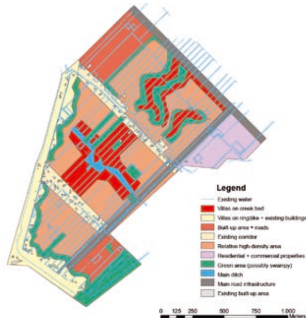
Figure 36: Overall picture of the compartmentalization method, incorporating the raised N219 and including the existing watercourse structure
