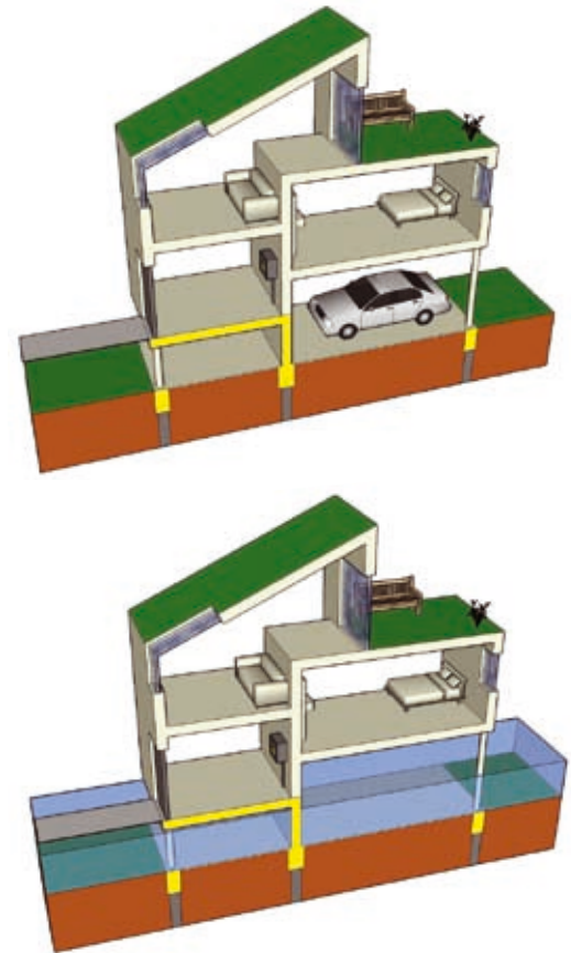
Figure 40: Climate resilient design: wetproof split level
