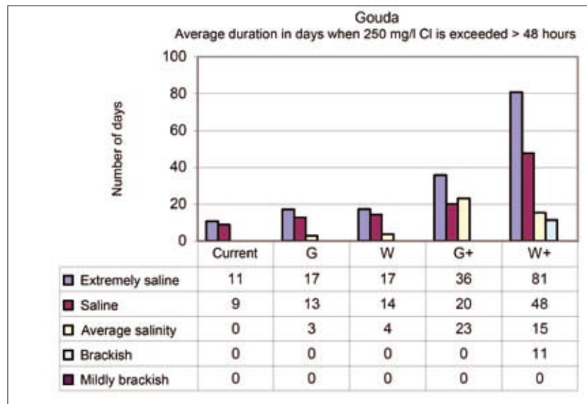
Figure 12: Average duration in days that 250 mg/l Cl is exceeded for longer than 48 hours at Gouda (Source: Beijl, 2008)
